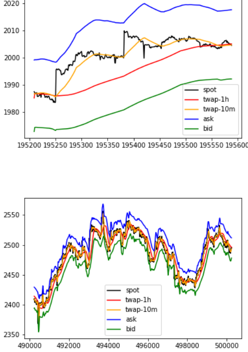
FIG. 5: Plots of the bid-ask spread around 1h and 10m rolling TWAPs against the same set of simulated data as Fig. 4. Static spread on the more extreme end of \delta = 0.00625 has been applied. Front-running the spot jump at t = 195250 is no longer profitable. Zooming out with the bottom plot to look at 2 days of simulated data shows the market remains tradeable.
