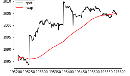
FIG. 4: Plot of the 1 hour rolling TWAP against spot price for Monte Carlo simulated 10m data generated from WETH/USDC fits. The jump in spot is not fully realized in the value of the 1h TWAP until one hour after it occurs.
