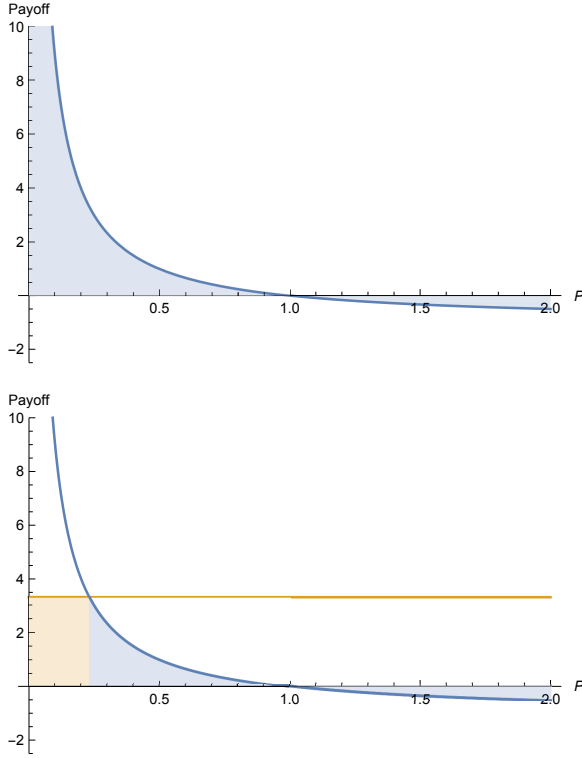
FIG. 7: Plots of the inverse market payoff with and without a cap as a function of price P , normalized with respect to the initial price at entry. P is the number of ETH per OVL. Without the cap, a single position could print an infinite amount of OVL. The payoff cap (orange line), however, eliminates this possibility by limiting the damage for each trade. For an ETH/OVL market, Uniswap V3 price ratio used would be y/x where y is the number of OVL virtual reserves in the pool and x is the number of ETH virtual reserves (i.e. 1/P ).
